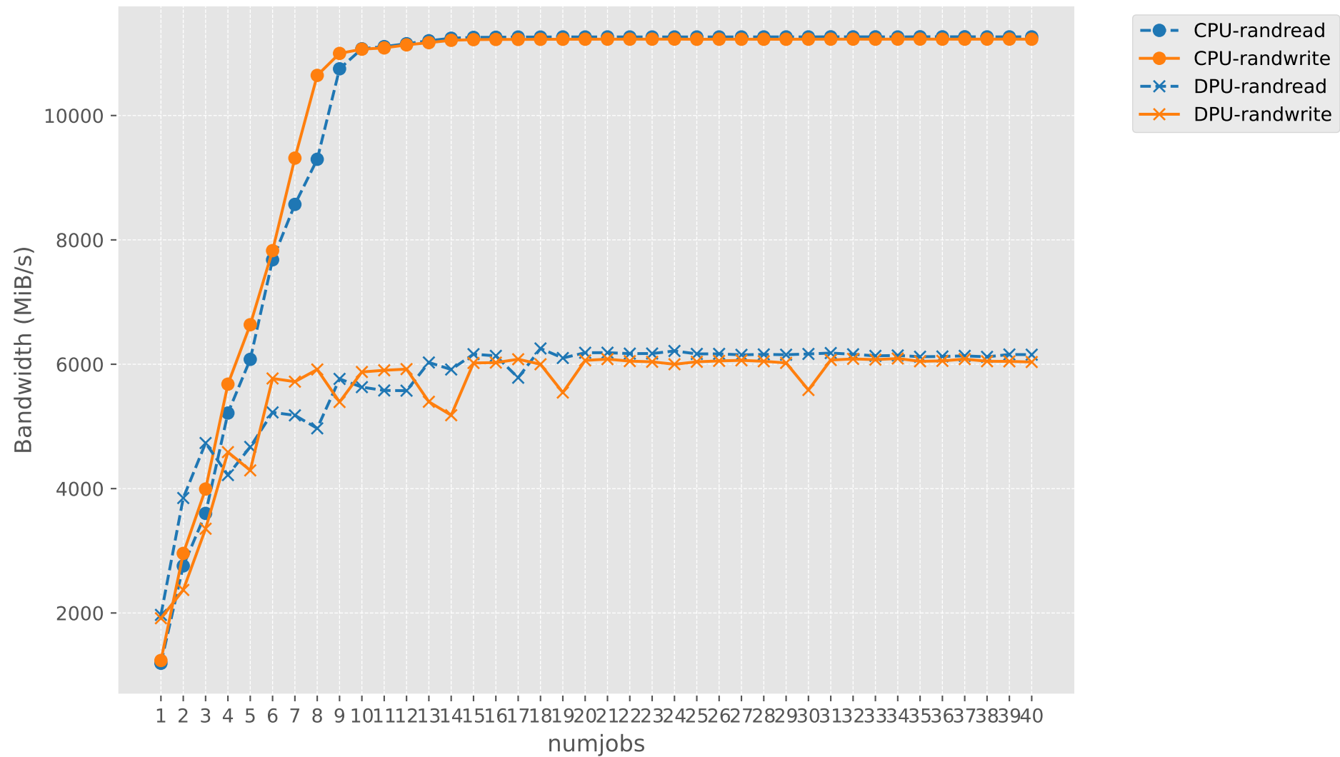
Bandwidth vs numjobs (CPU vs DPU)
